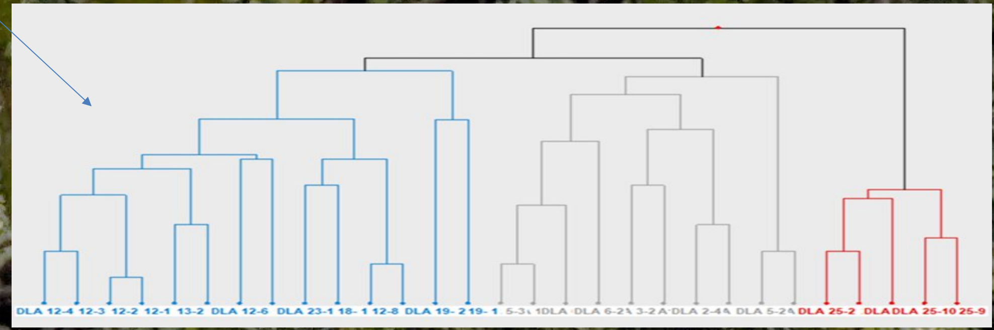
Dendrogram of accessions in germplasm bank
